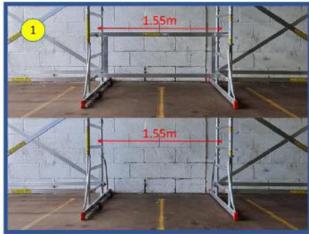
Assemble tower bases and attach 1 x guard rail between them for spacing then remove.
